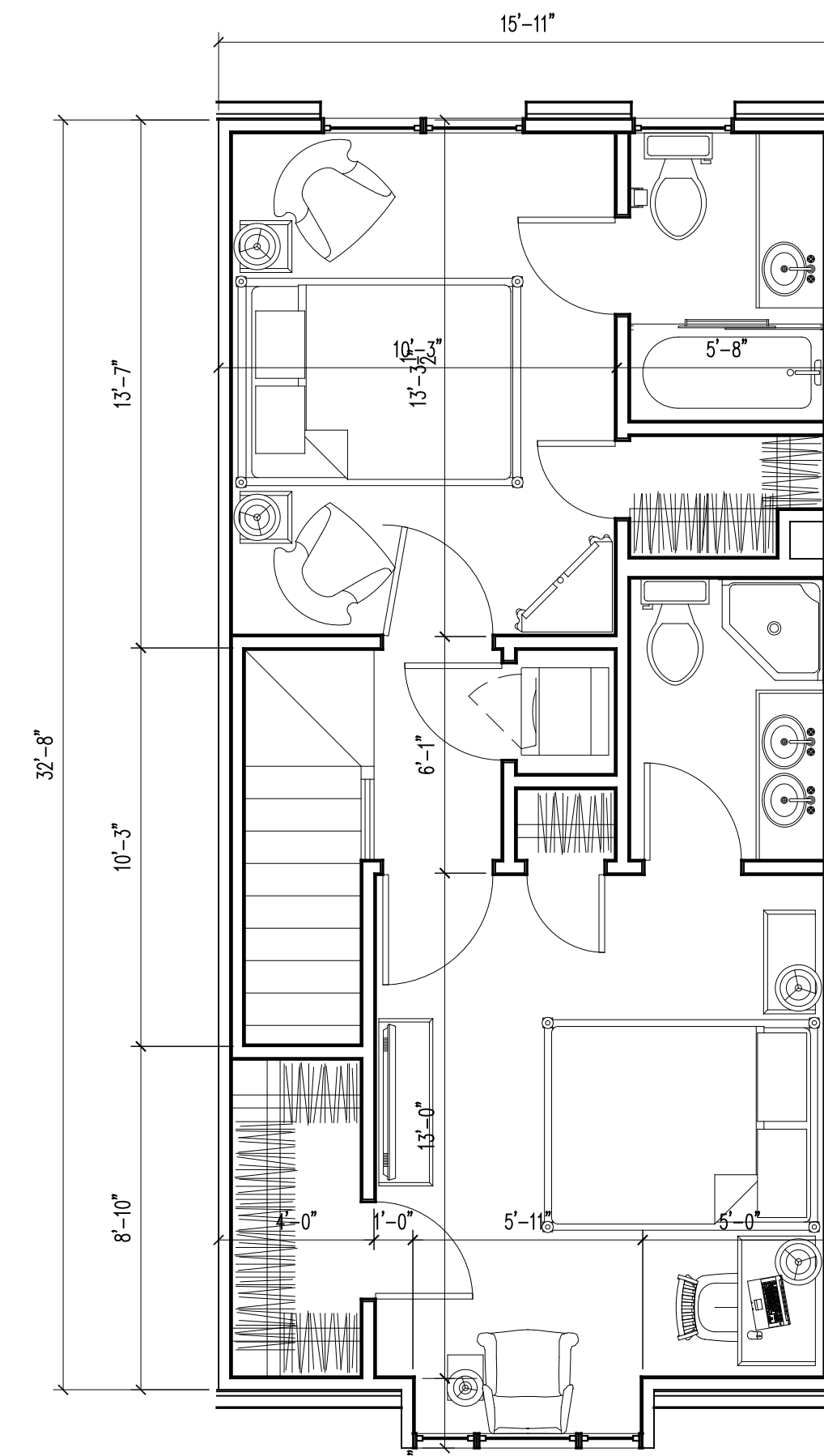
UPPER FLOOR
