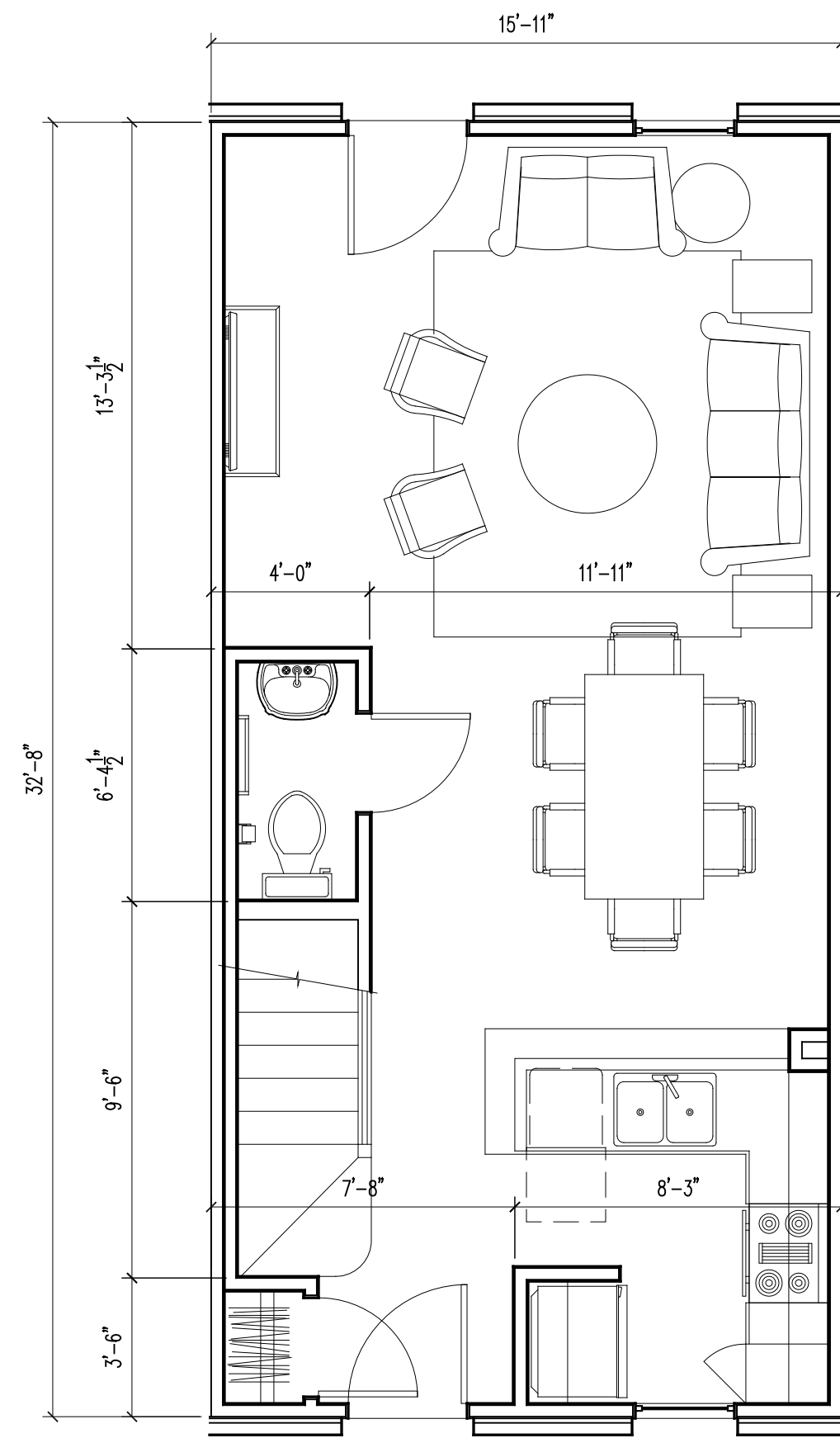
GROUND FLOOR
